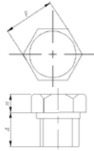
Hex Head Plug
