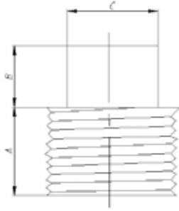
Square Head Plug
